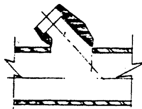
SOCKET WELDING
