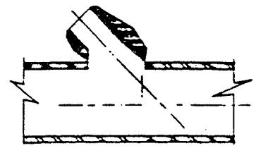
BUTT WELDING
